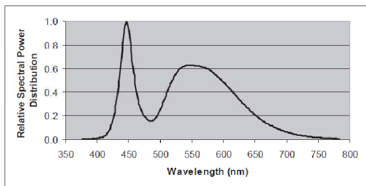
Cool-White at Test Current Thermal Pad Temperature = 25°C
