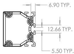
DETAIL A SCALE 1 : 2
