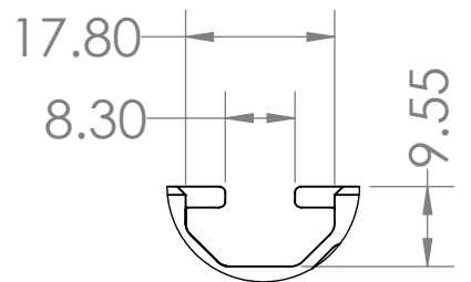
Mounting Rail DETAIL A SCALE 1 : 1
