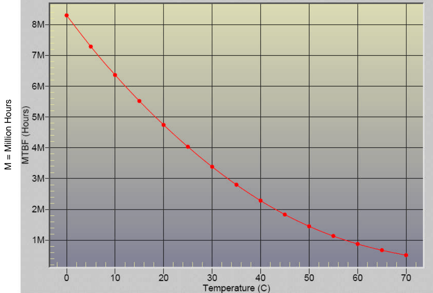
MTBF vs Temperature LED-DRIVER-BOM.CIR
